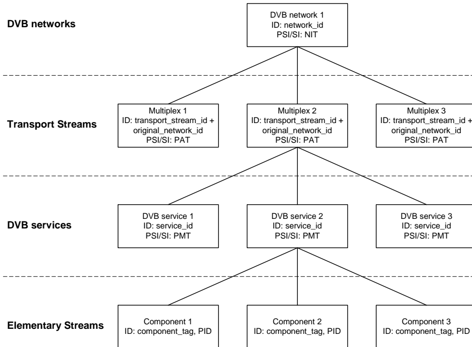
Figure 1: Hierarchy of data streams in DVB-H (1)
