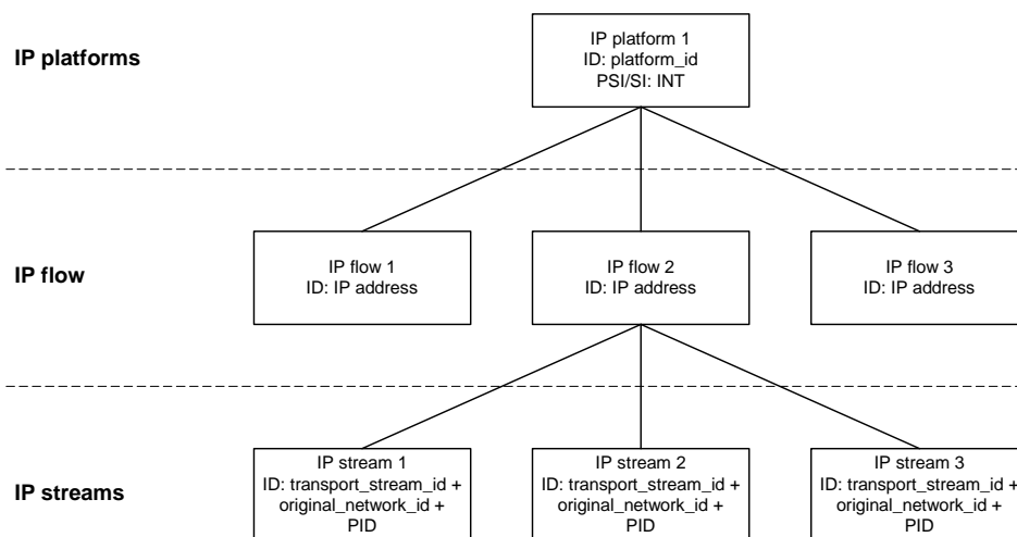
Figure 2: Hierarchy of data streams in DVB-H (2)
