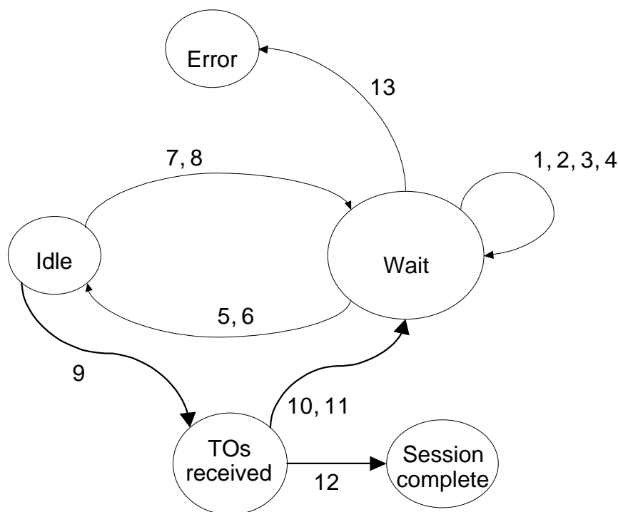
Figure 7: State machine
